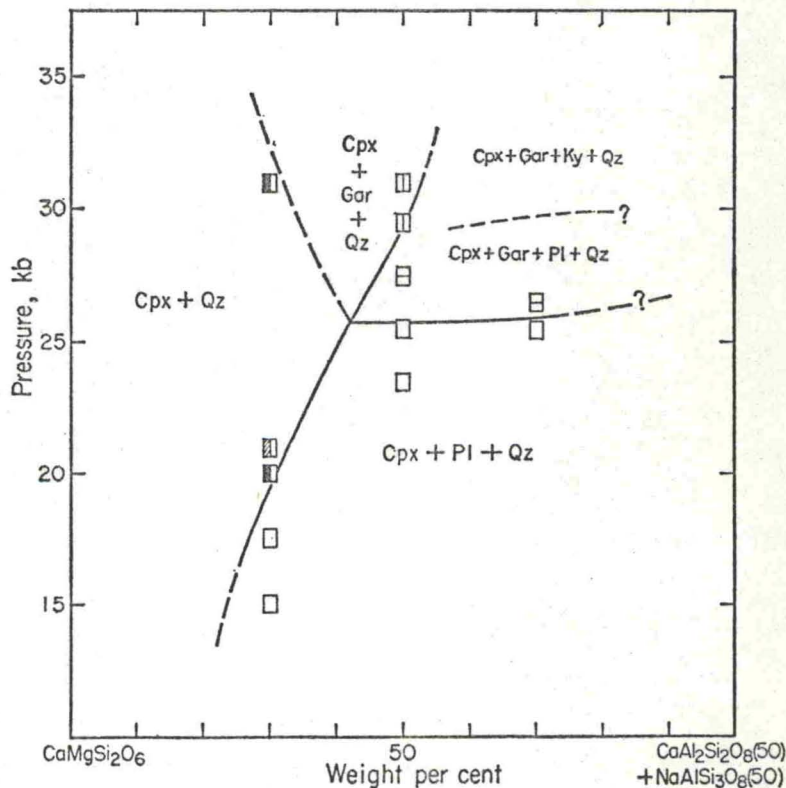
Fig. 17. Subsolidus phase-equilibrium relations on the join diopside-plagioclase (An 50 Ab 50 wt %) at 1150°C. Abbreviations: Cpx, clinopyroxene (diopside solid solution); Gar, garnet; Ky, kyanite; Pl, plagioclase; Qz, quartz.
